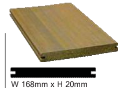
ROFILE Decking Solid 168 x 20 DB16820
